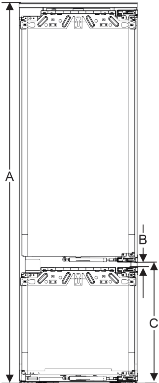
Fig. 69 Gap position for double-door unit front
