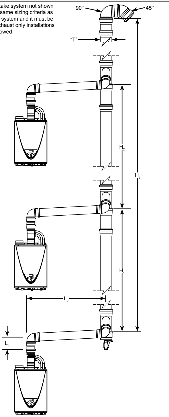
Figure 11. Vent Dimensioning
