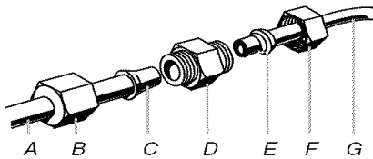
A. Water tubing B. Nut (provided) C. Bulb D. Coupling (provided) E. Ferrule (purchased) F. Nut (purchased) G.
