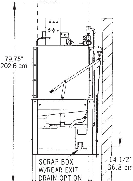
SIDE VIEW
