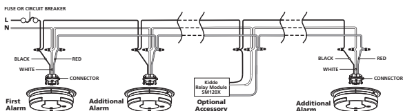
FIGURE 4 INTERCONNECT WIRING DIAGRAM
