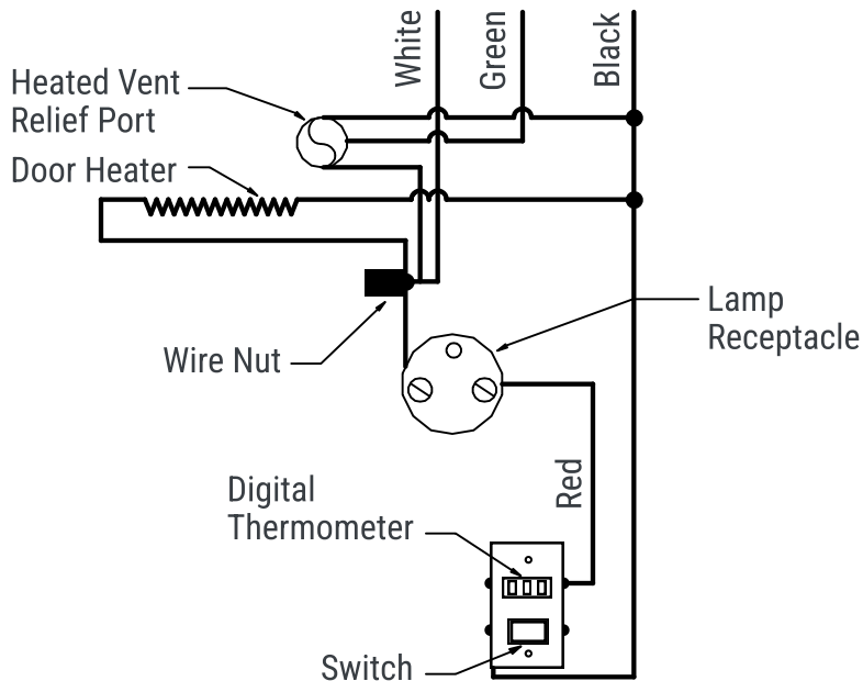
WIRING DIAGRAM
