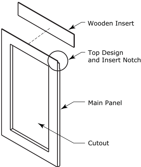
Integrated Frame
