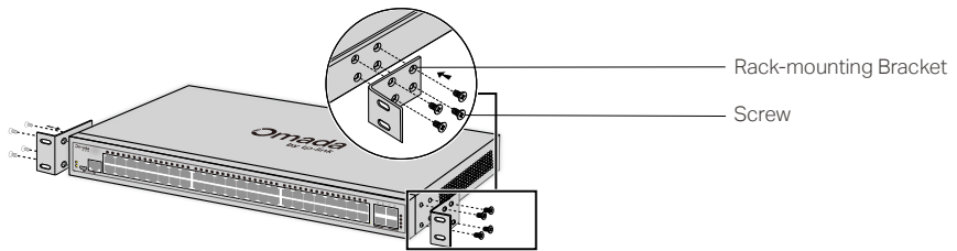
Figure 2-2 Bracket Installation
