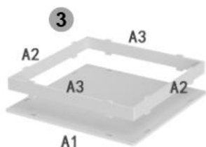
3 A1+A2+A3 assembled together
