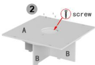
2 Assembly completed the whole flip
