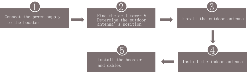
Flow chart of LCD Assisted Install
