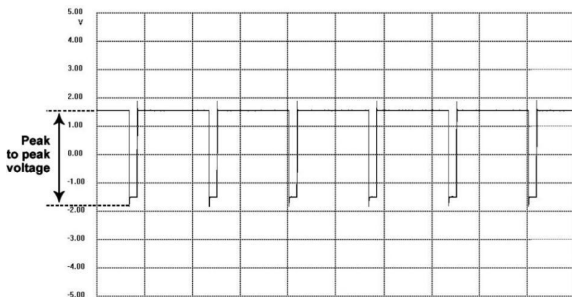
Figure 15-2 Sample Square Waveform
