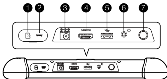
Figure 2-3 Display Tablet Top View
