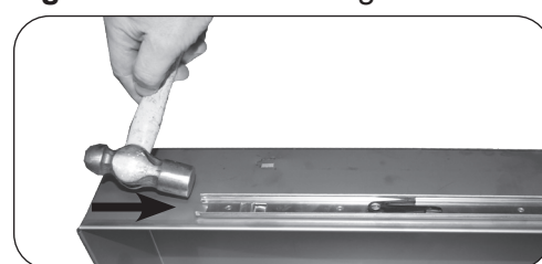
Fig. 5-4 Reinstall runners
