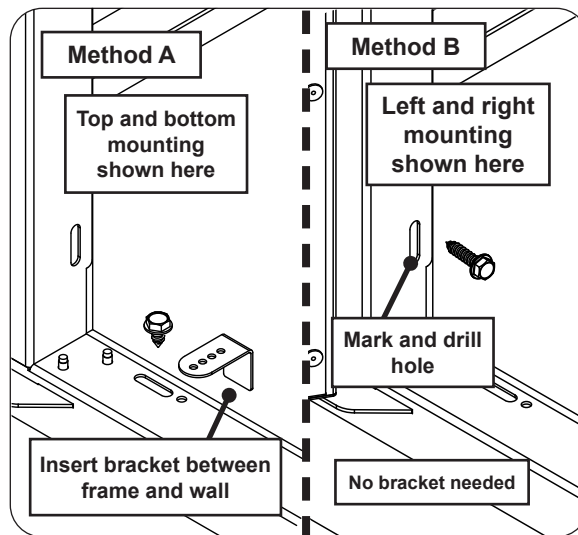
Fig. 2-3 Installation methods
