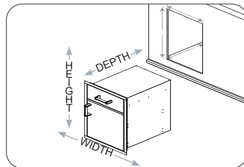
Fig. 5-1 Pantry cut-out diagram
