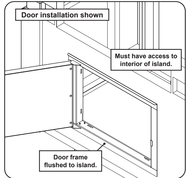
Fig. 3-1 Insert door/drawer/pantry
