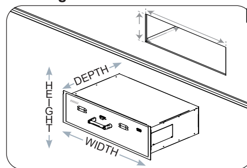
Fig. 5-5 Drawer cut-out diagram
