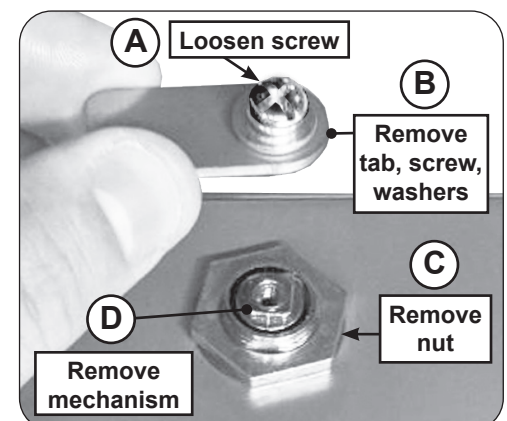
Fig. 4-5 Locking / unlocking
