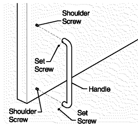
Typical Handle
