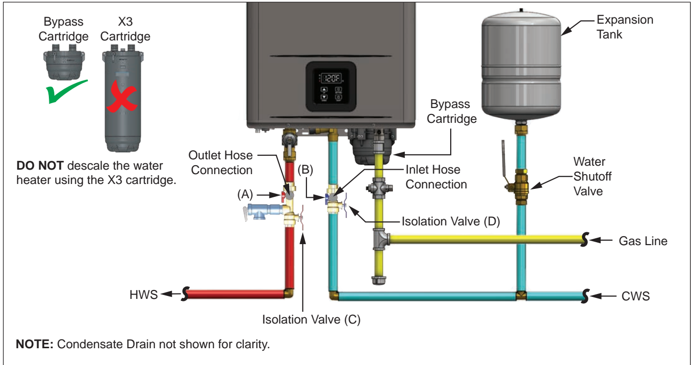
Figure 6 - Descaling the water heater
