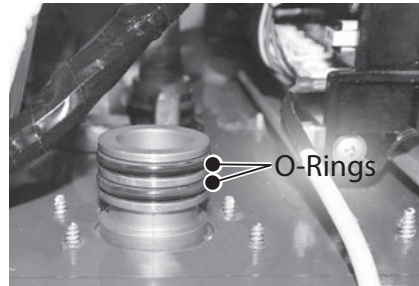
Figure 93 - Gas connector O-rings
