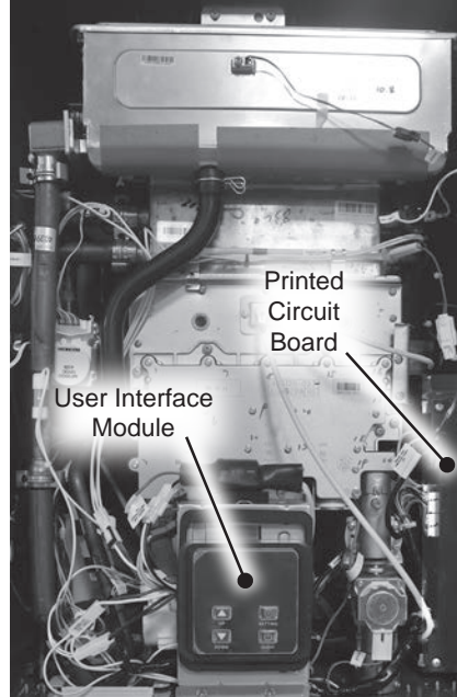
Figure 13 - Locating UIM
