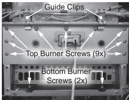
Figure 160 - Burner screws and guide clips
