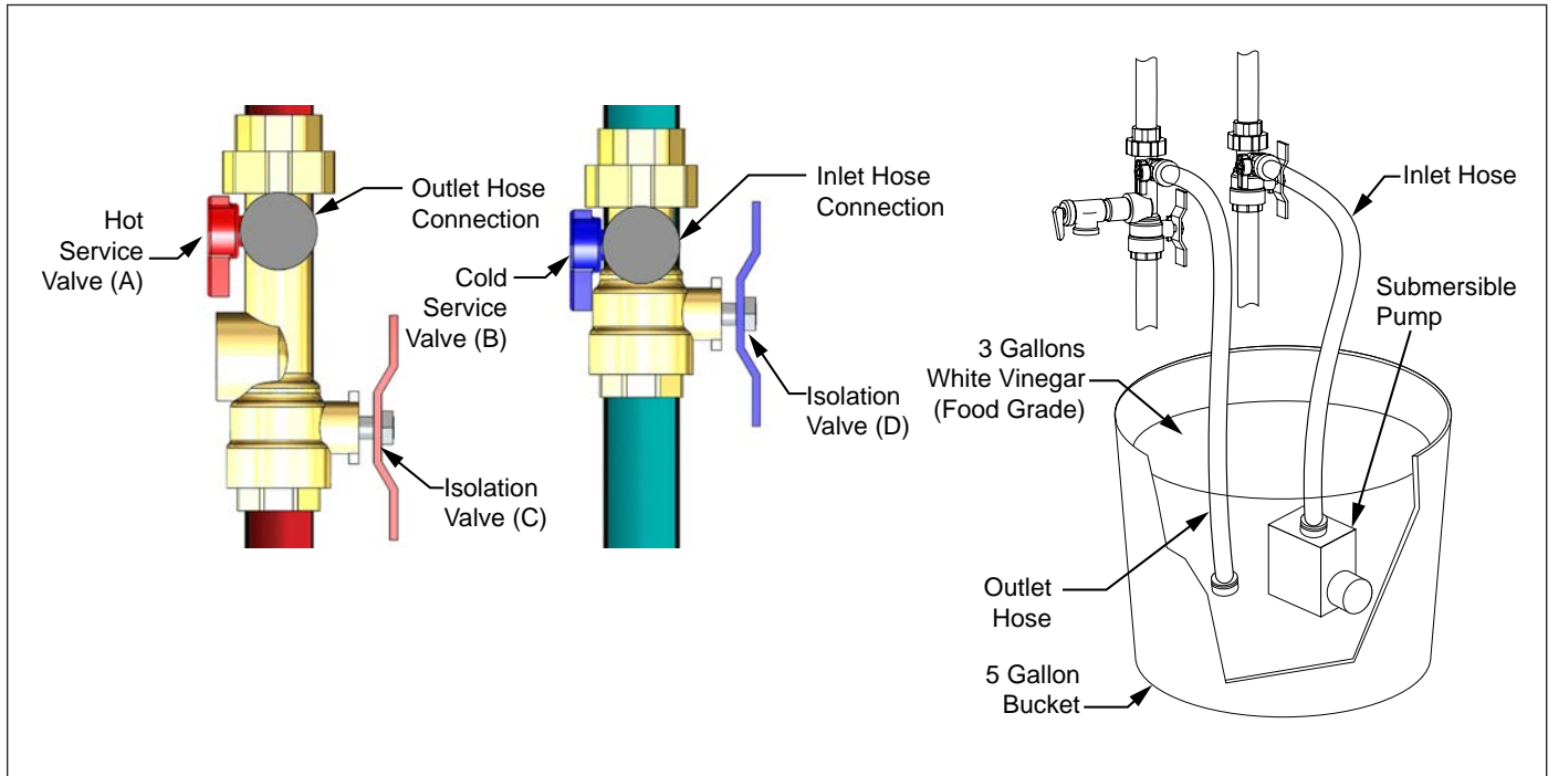
Figure 7 - Isolation valve connection points
