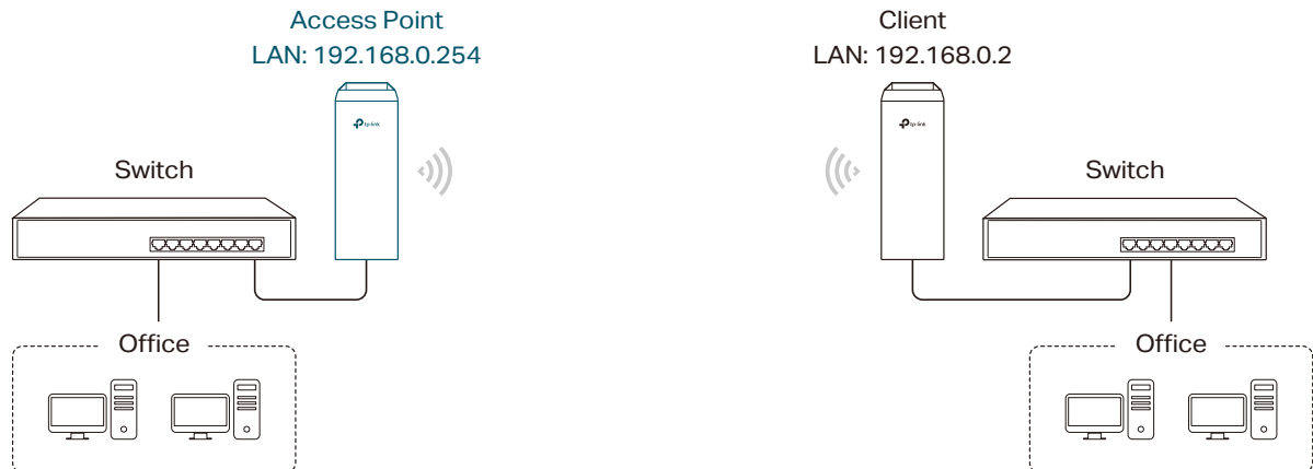
Figure 1-2 Scenario Two for Access Point Mode
