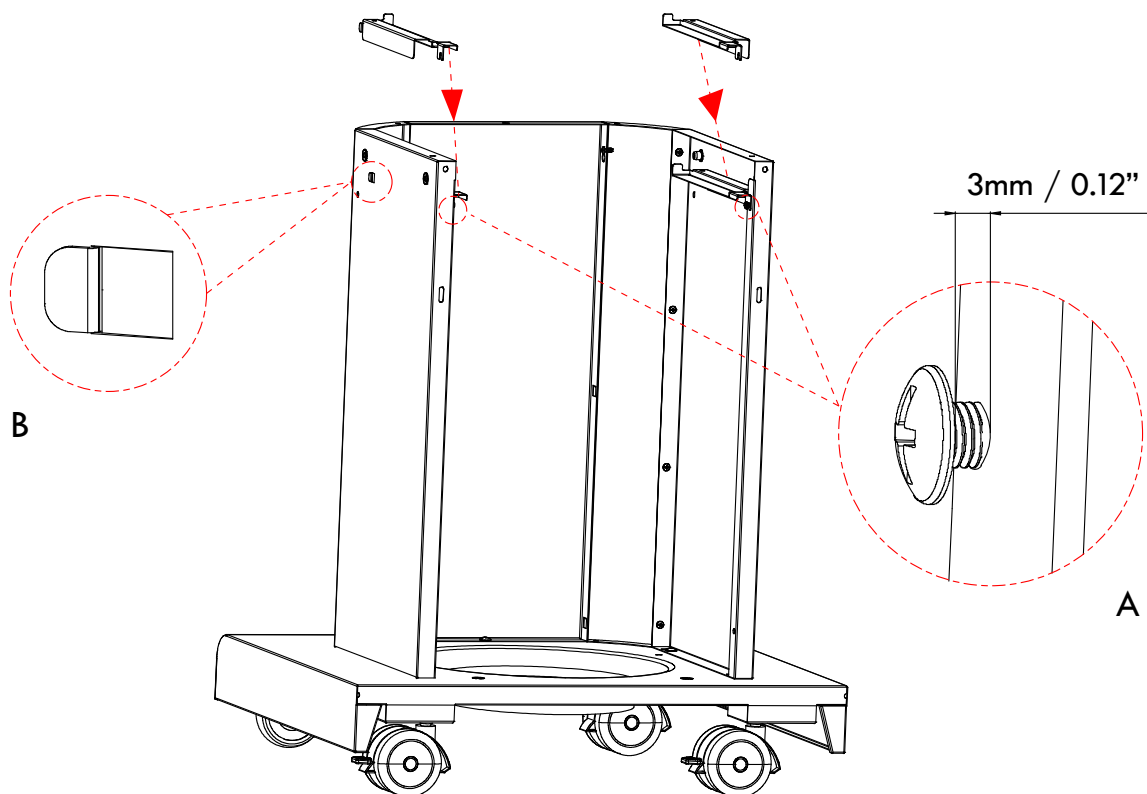
M4x10 Screw Qty: 2 pcs
