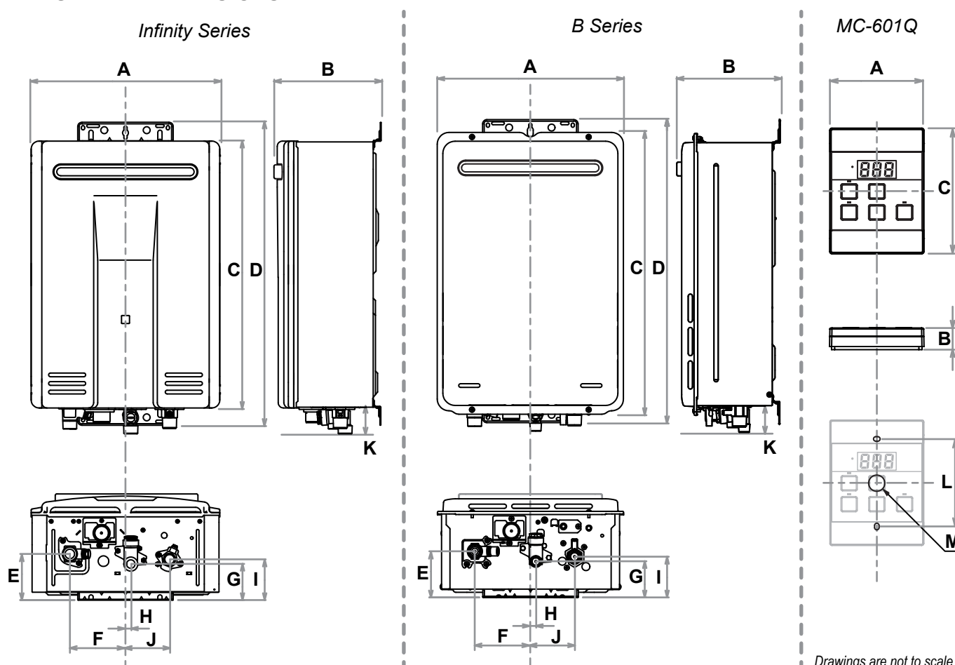
DIAGRAM 1. DIMENSIONS
