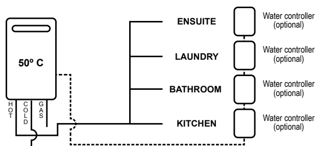
Diagram 1 : 50°C Appliance
