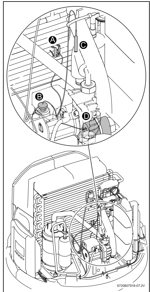
Fig. 19 Sensor positioning
