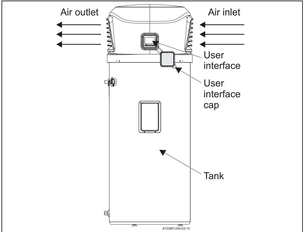
Fig. 3 Appliance overview
