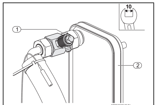
Fig. 16 Purge valve
