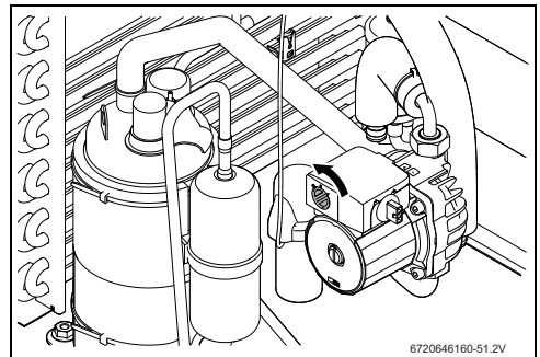
Fig. 15 Circulation pump
