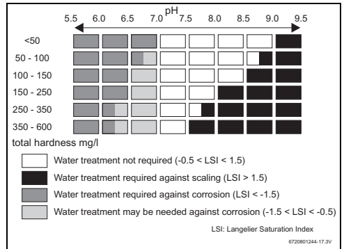
Fig. 18 Water treatment vs water characteristics
