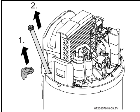
Fig. 60 Check state of magnesium anode
