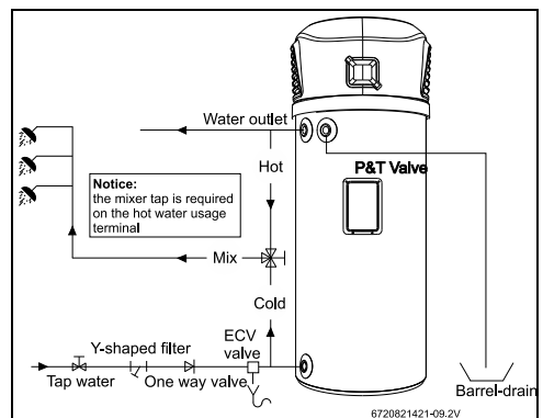
Fig. 9 Typical installation
