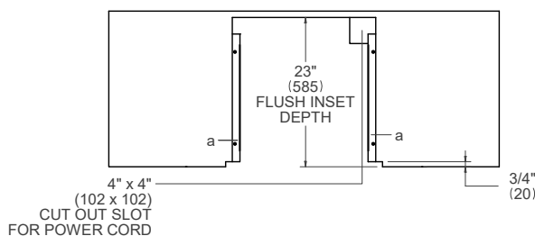
TOP VIEW – OVEN DETAIL
