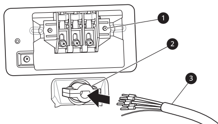
1 Terminal Block
