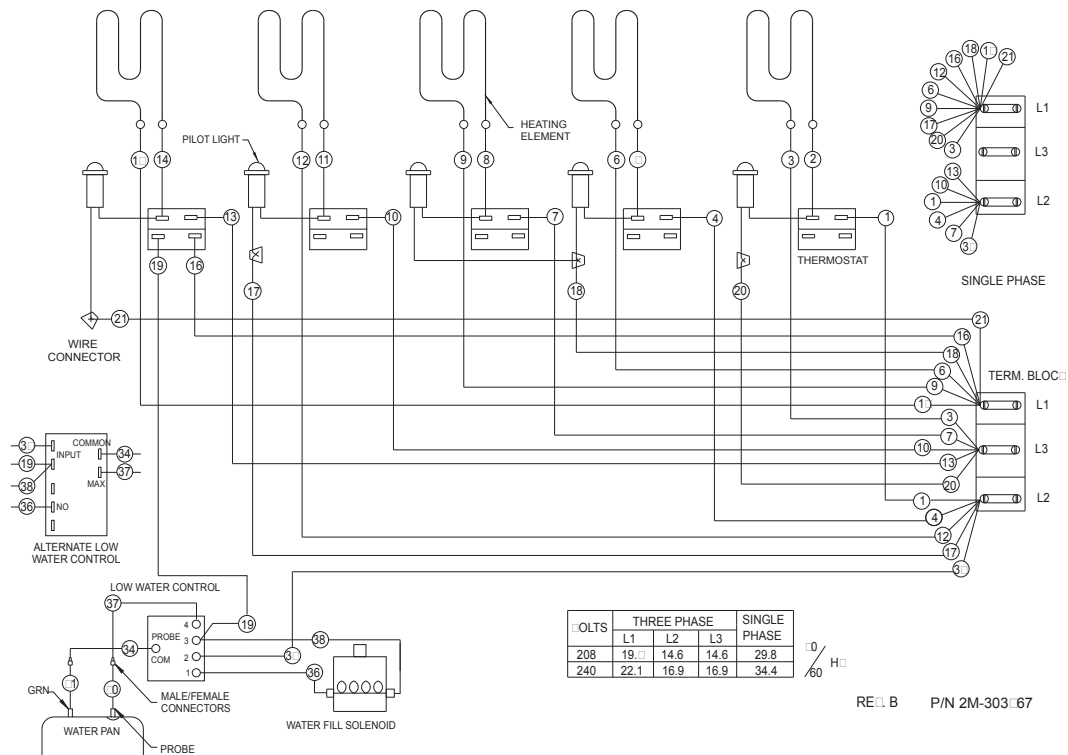
WIRING DIAGRAM FOR MOD-00TDM, 027TDM W/AUTO WATER FILL (SINGLE CONTROL PANEL) 208/240V, SINGLE □ THREE PHASE
