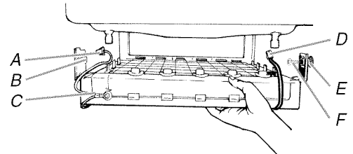
A. Cutter grid harness B. Screw C. Cutter grid D. Ice level sensor harness E. Plastic spacer F. Screw
