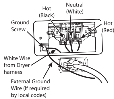
Three-wire connection for electric dryers: Power cord
