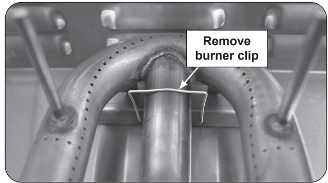
Fig. 41-1 Main burner removal
