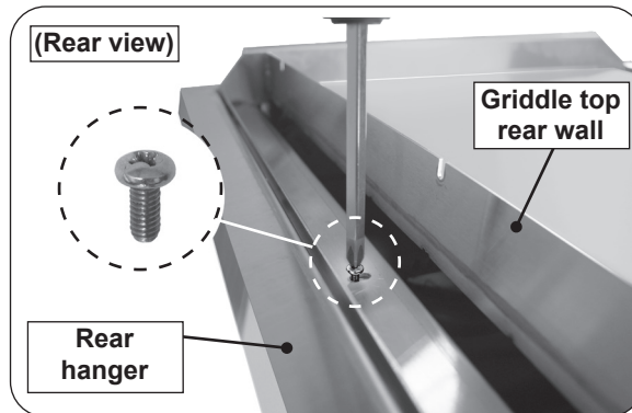
Fig. 32-3 Secure griddle top
