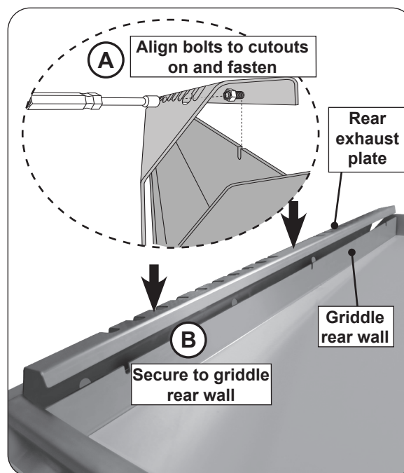
Fig. 32-4 Install rear exhaust plate
