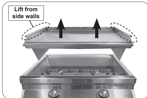
Fig. 28-2 Remove griddle top
