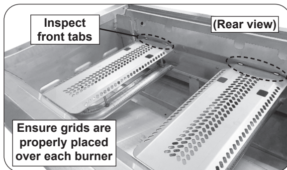
Fig. 32-1 Inspect heat distribution grids
