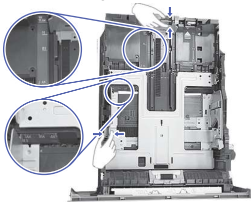
Figure 9-19 Adjust guides
