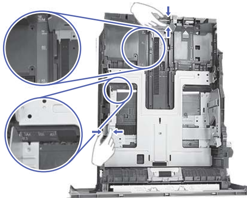
Figure 9-14 Adjust guides
