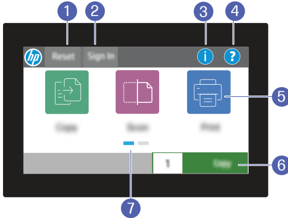
Figure 1-8 Color touchscreen control panel
