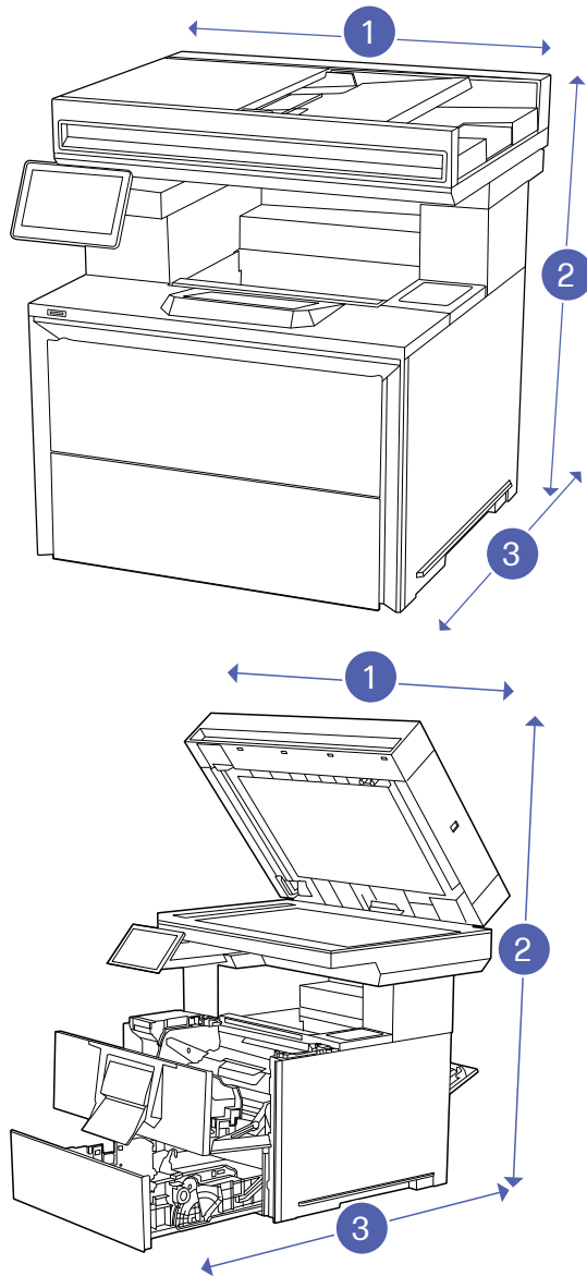
Figure 1-9 Printer dimensions
