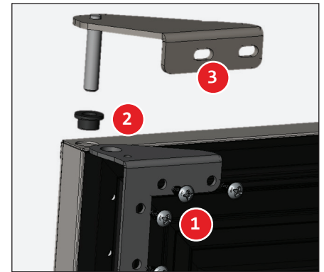
Fig. 7b. Top hinge component assembly.
