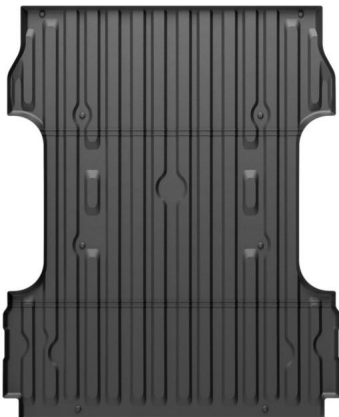
Model: F250-F350-6,8ft
