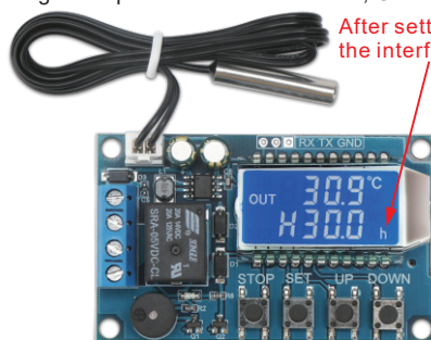
DC 6.0~30V Wiring Method
