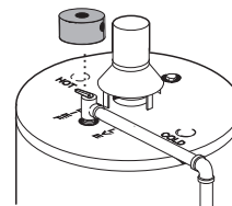
Typical Top Connect T & P Arrangement.
