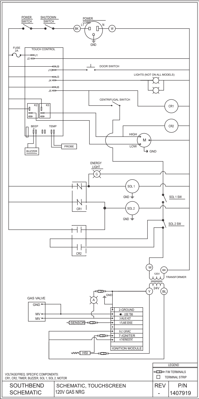
Wiring Diagram for 120 Volt Gas NRG Touchscreen Models
