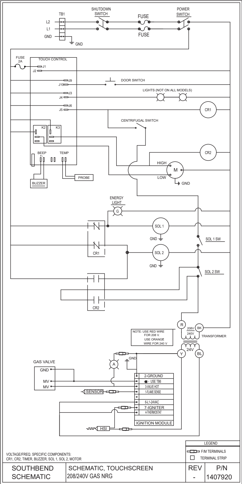
Wiring Diagram for 208-240 Volt Gas NRG Touchscreen Models
