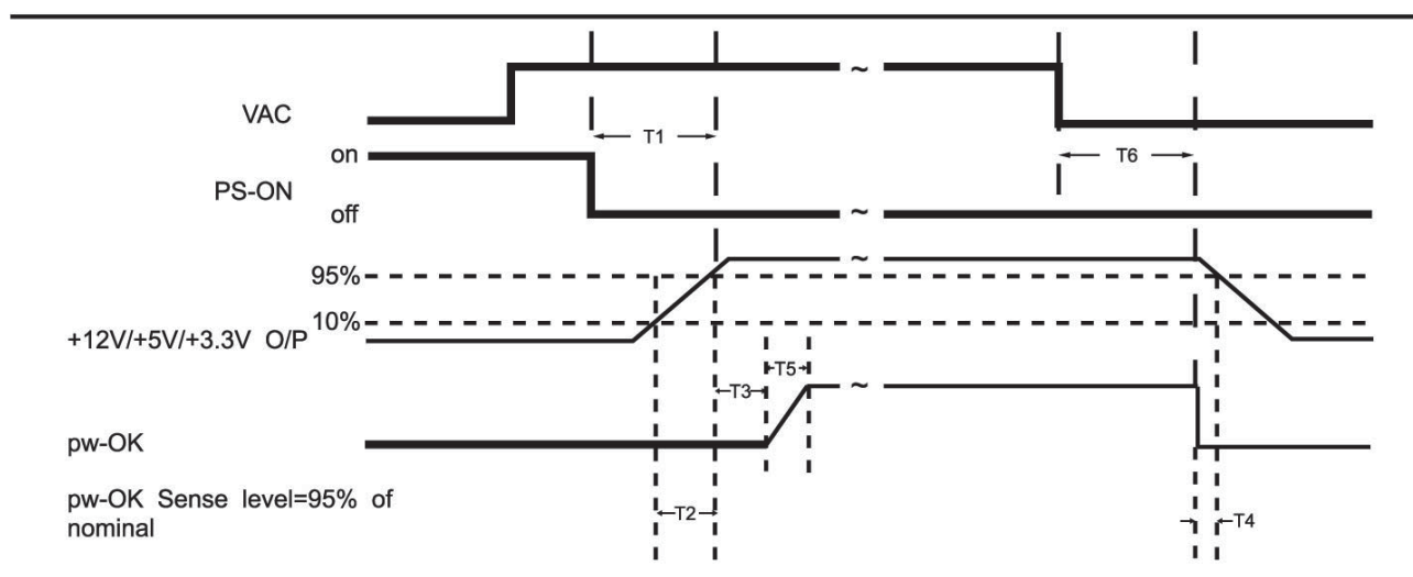
Figure 2. PS-OK Timing Sequence
