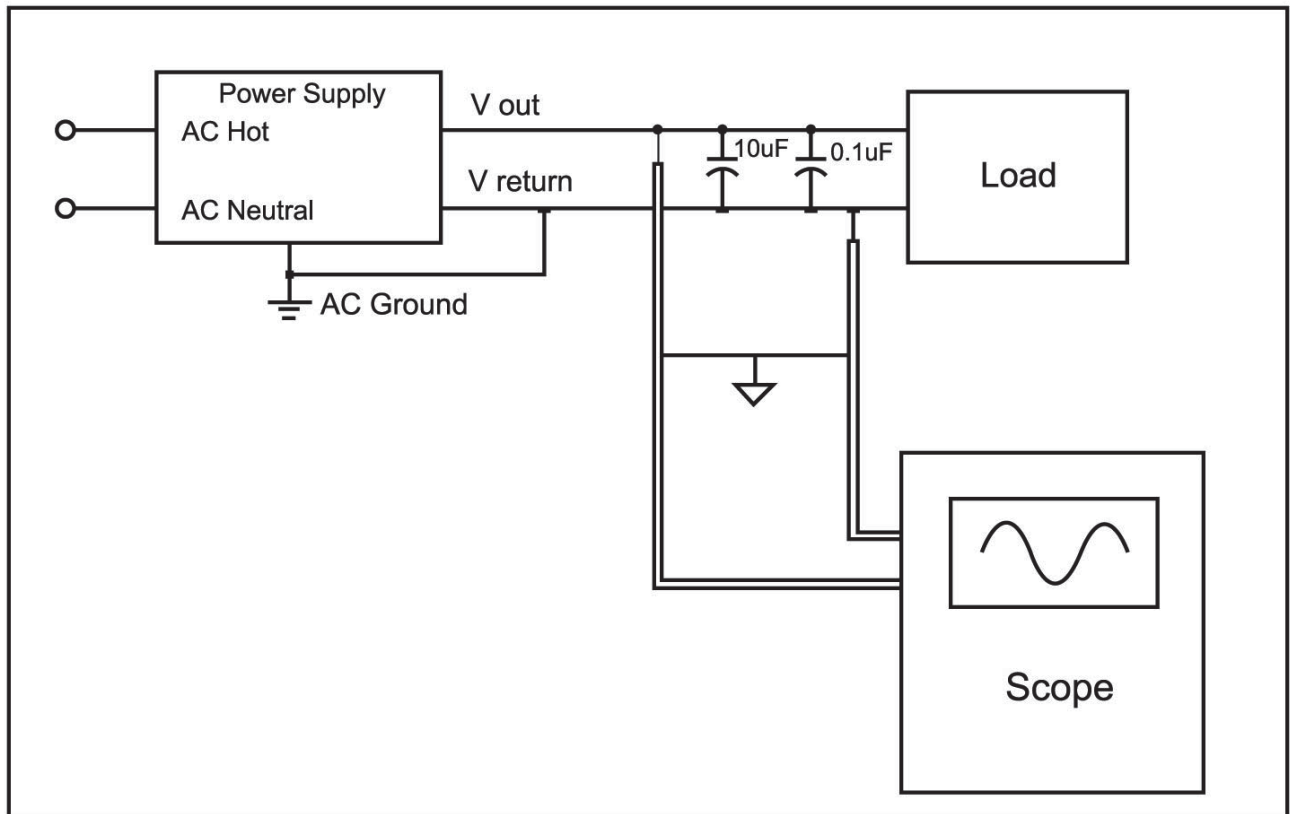
Figure 1. Ripple voltage test circuit
