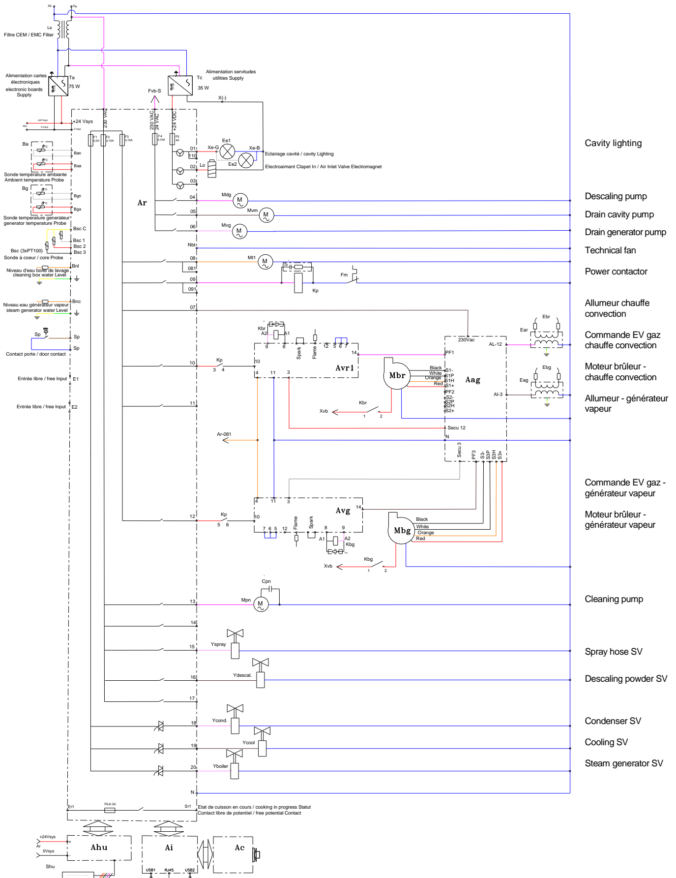
Wiring diagram
