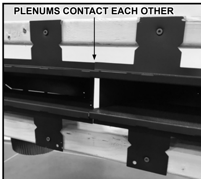
Figure 5.21 Plenums Contact Each Other
