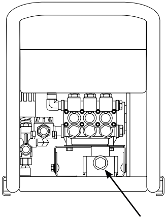
Pump tensioner
