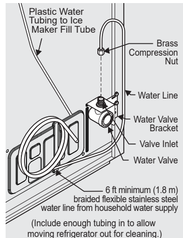
Units with braided flexible stainless steel tubing
