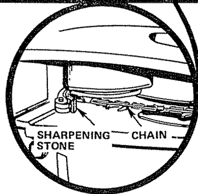
VIEW FROM BOTTOM OF SAW ON ITS LEFT HAND SIDE
