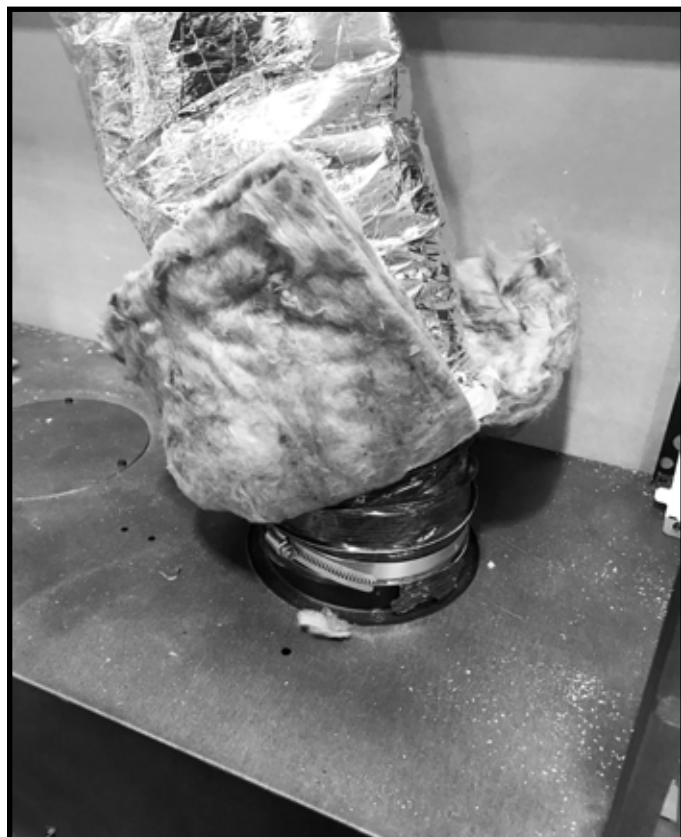
Figure 5.27 Install Flex Venting to Appliance
