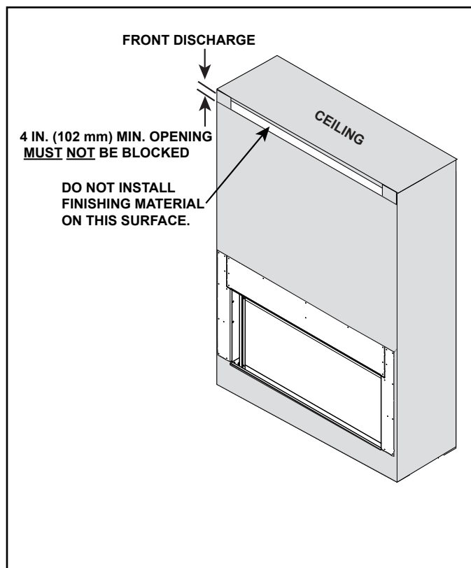
Figure 5.32 Finishing Material Installed
