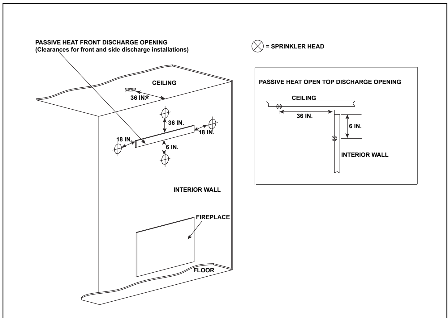
Figure 3.1 Sprinkler Head Clearance
