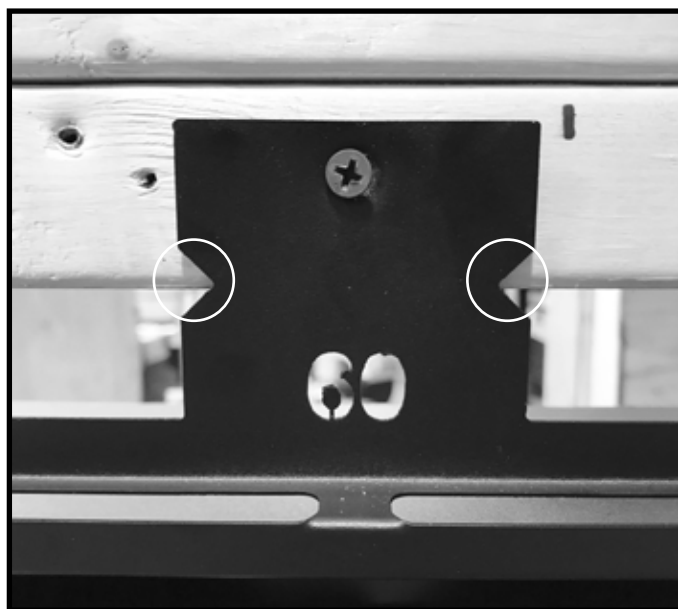
Figure 5.19 Secure Nailing Tabs
