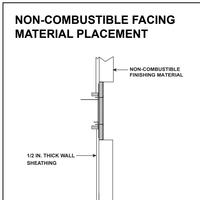
Figure 5.31 Finishing Material Installed
