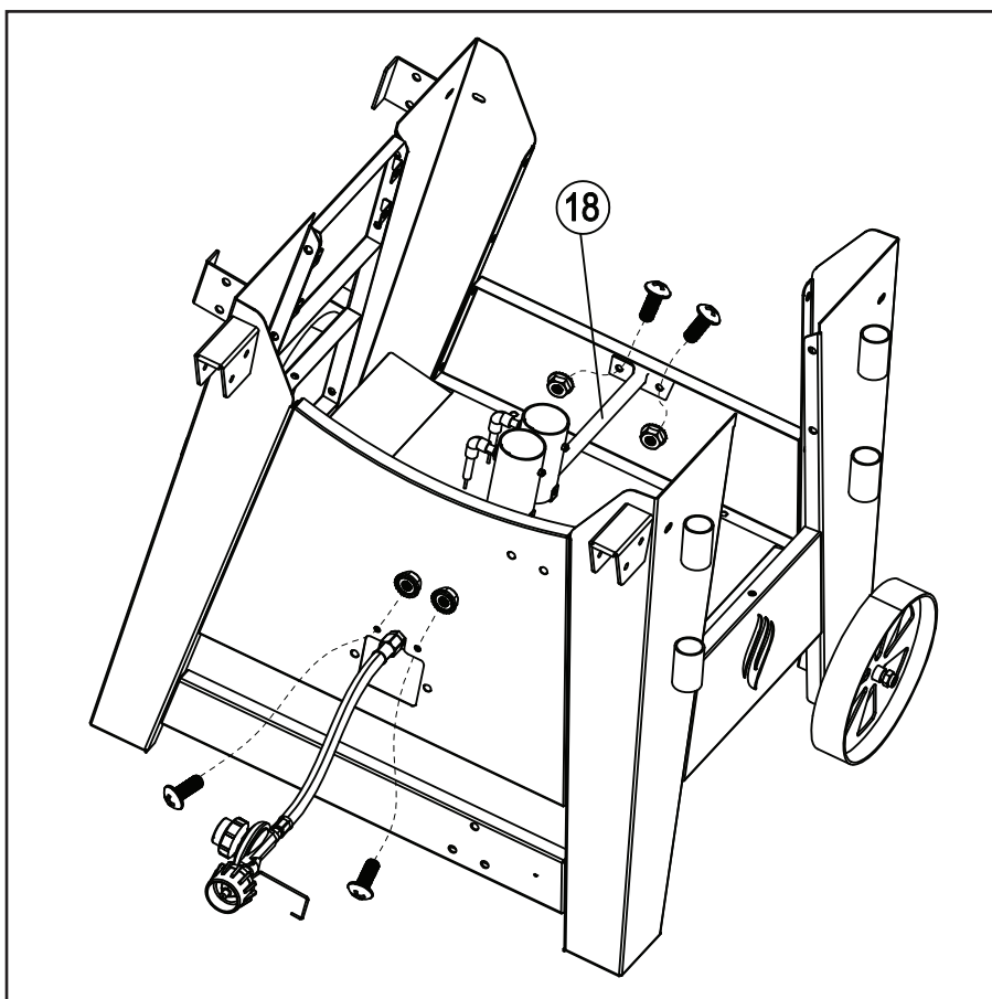
Burner Assembly (90 Qt. or 150 Qt)
