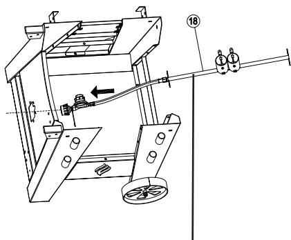
Burner Assembly (90 Qt. or 150 Qt)
