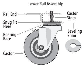
Fig. 7. Install shim(s).
