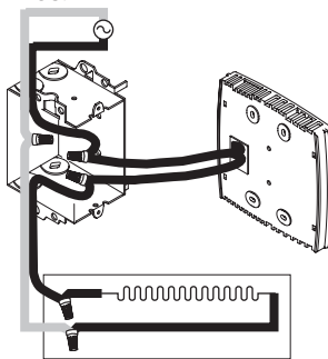
4-wire Installation
