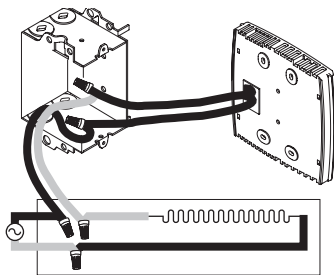
2-wire Installation
