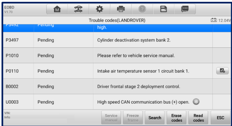
Figure 4-25 DTC & FFD Menu Screen
