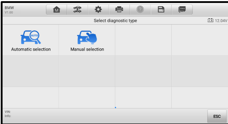
Figure 4-10 Selection Screen
