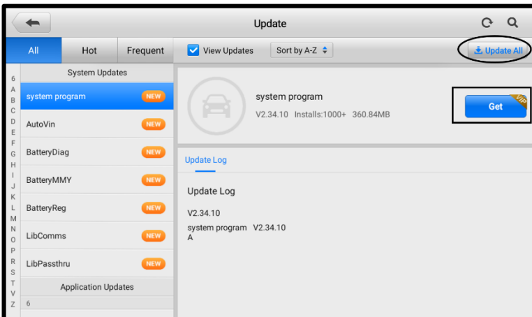
Figure 9-2 Update Screen 2
