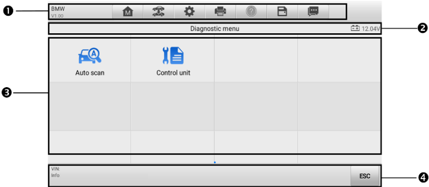
Figure 4-11 Diagnostic Screen
