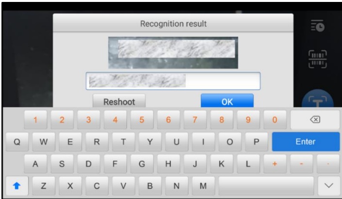
Figure 4-8 Scan VIN/License 2
