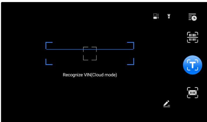
Figure 4-7 Scan VIN/License 1
