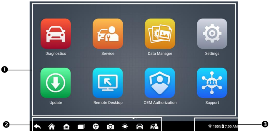
Figure 3-1 Job Menu
