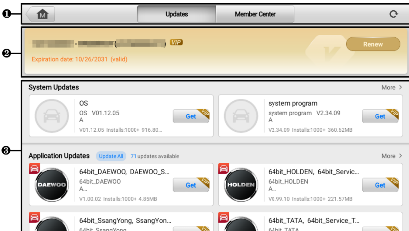
Figure 9-1 Update Screen
