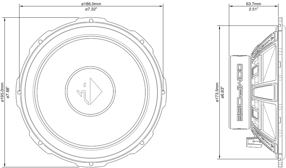
Speaker without adaptor ring
