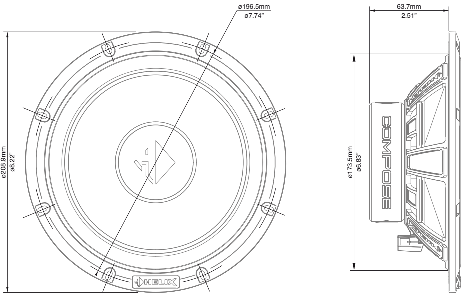
Woofer with assembled universal mounting ring
