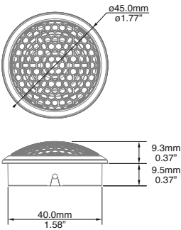
With housing for flush mount
