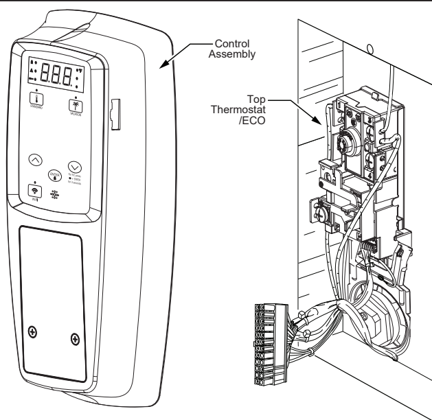
Figure 21 - Control Assembly
