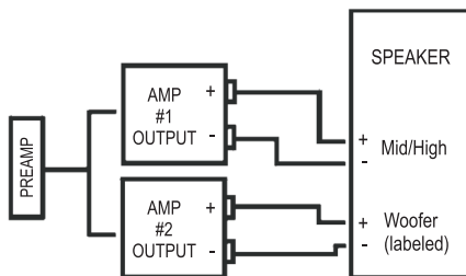
Figure 2: Bi-wire and Bi-amp Wiring Between Speakers and Amplifier
