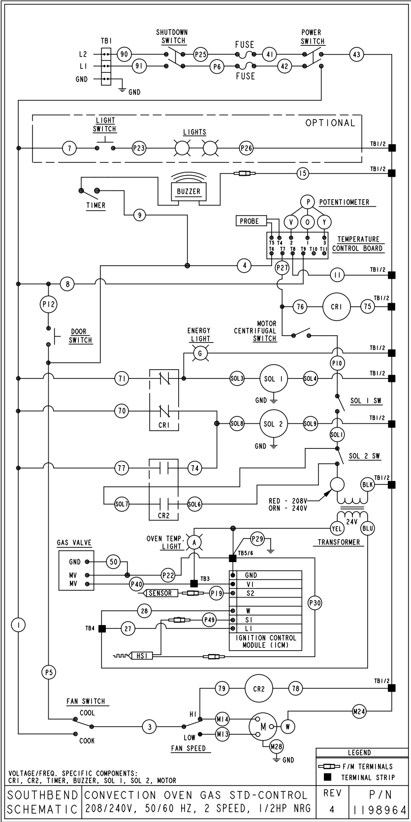
Figure 33 Wiring Diagram for 208-240 Volt Models with Standard Controls
