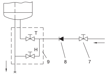
Fig. 3: Open (non-pressure) system
