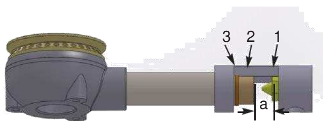
Orifice for gas oven
