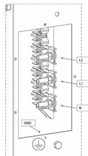
Terminal block
