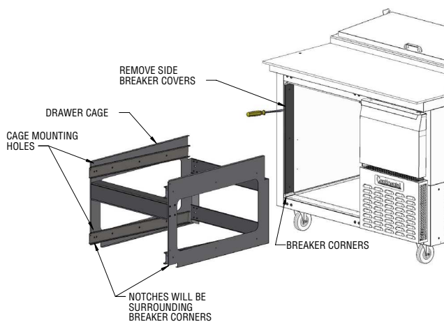
FIGURE 13: Drawer Cage
