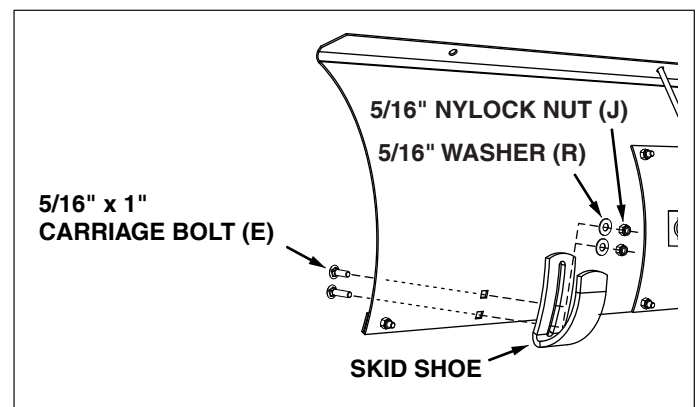
FIGURE 20 (Left Hand Side View)
