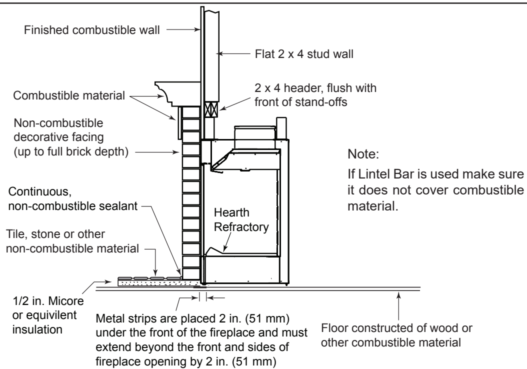
Figure 11.9 Decorative Facing
